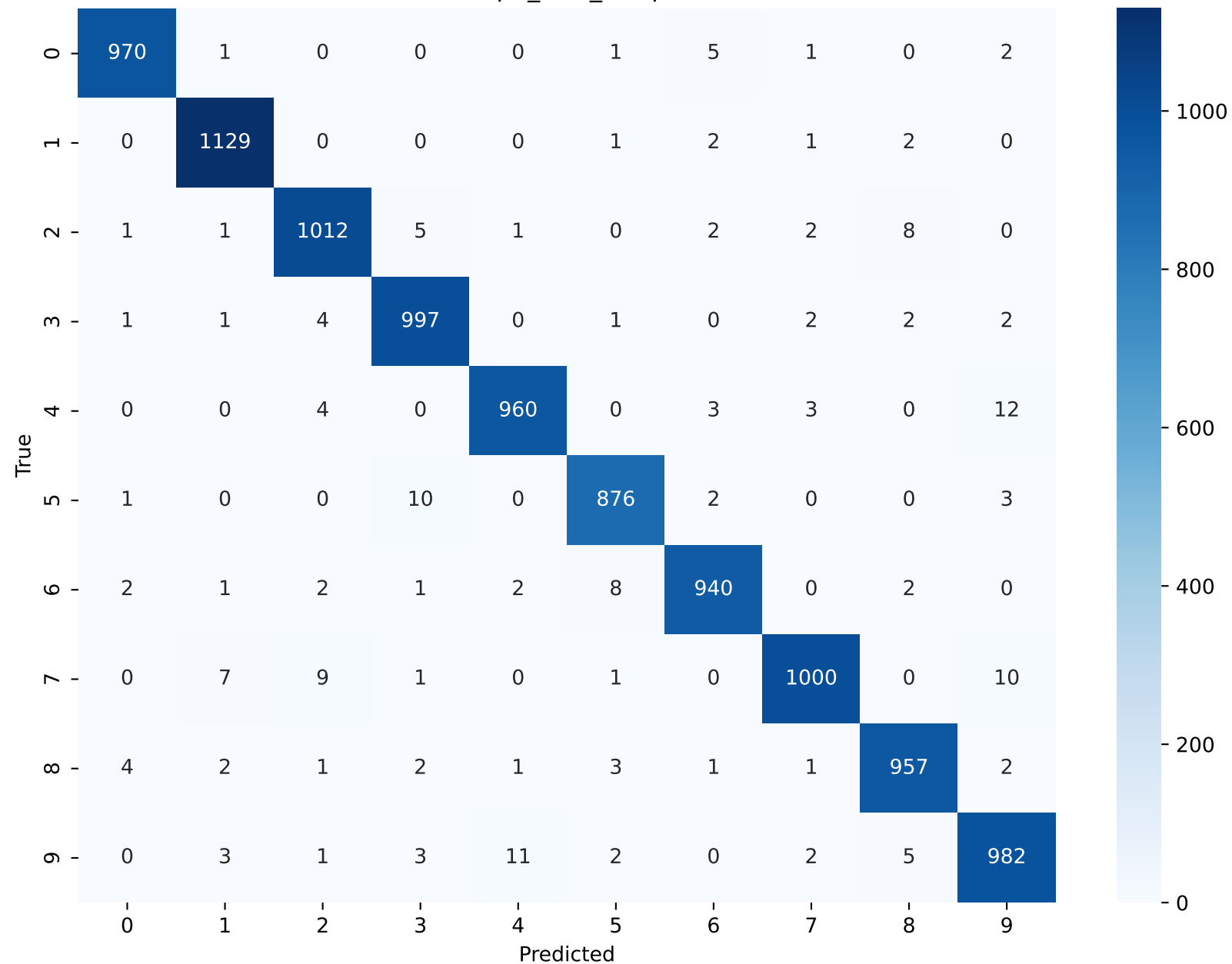
exp1_MLP_Deep
