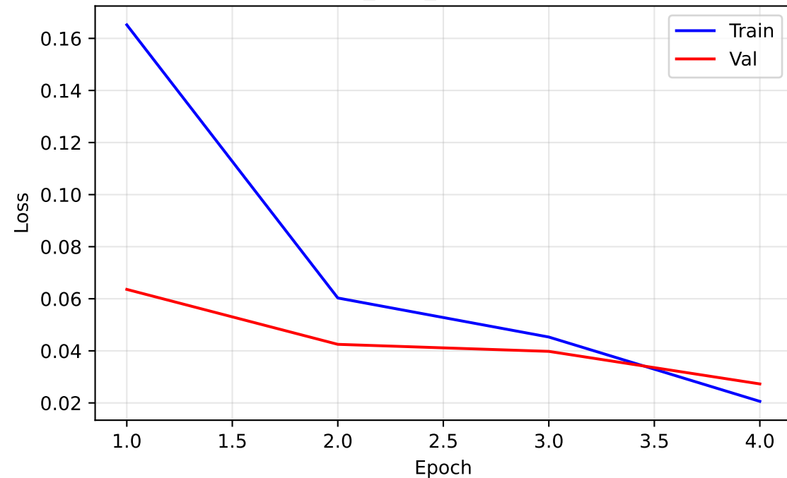
exp1_CNN_Better - Loss
