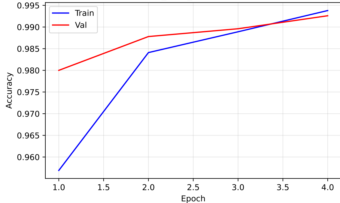
exp1_CNN_Better - Acc
