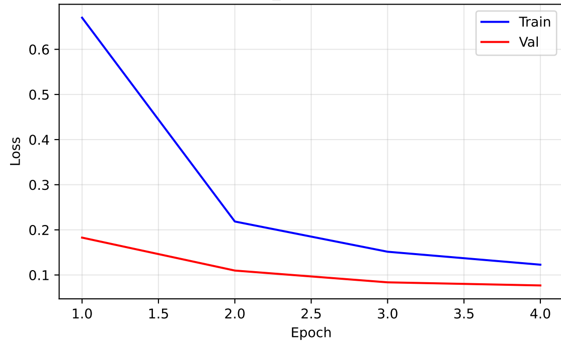
exp3a_lr0.0001 - Loss
