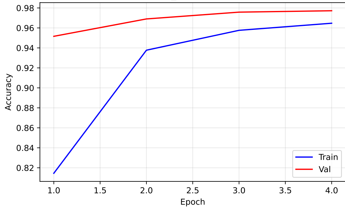
exp3a_lr0.0001 - Acc
