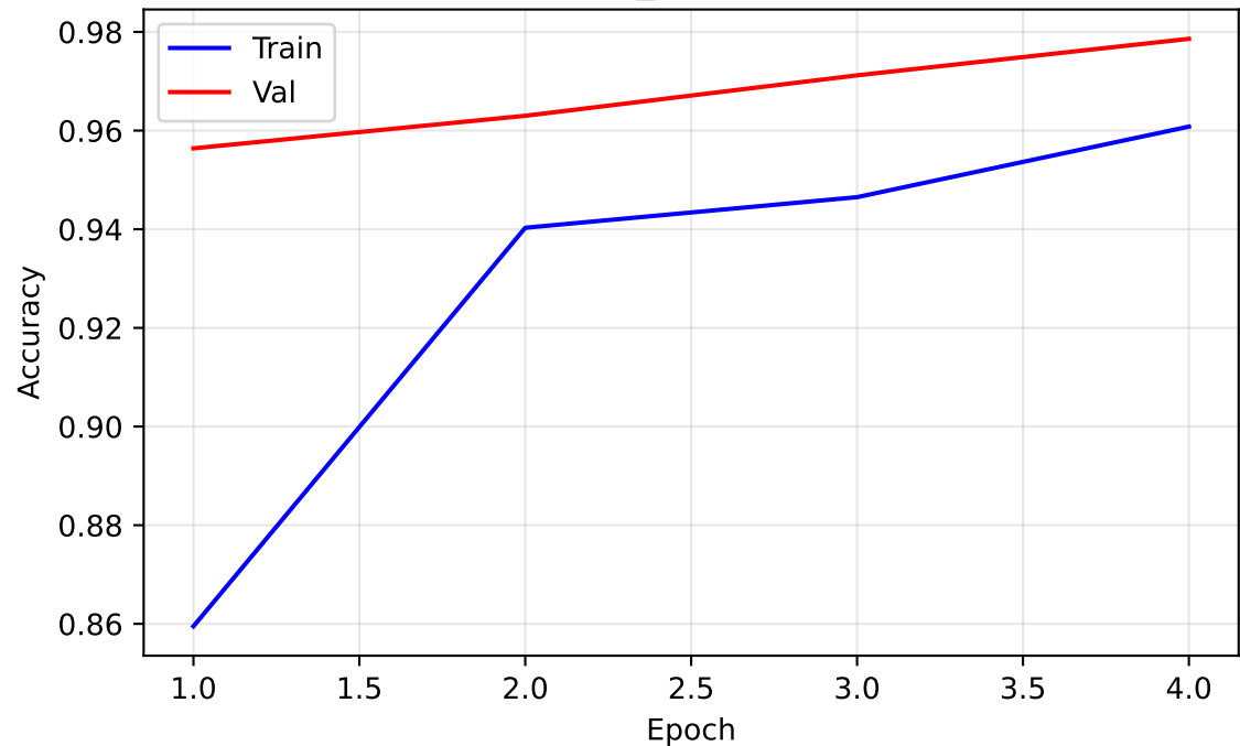
exp3a_lr0.01 - Acc
