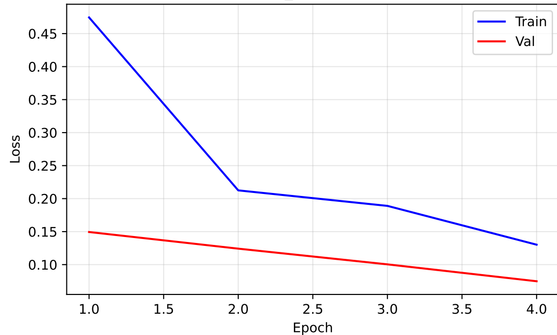
exp3a_lr0.01 - Loss
