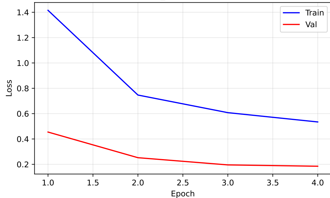
exp4_drop07 - Loss
