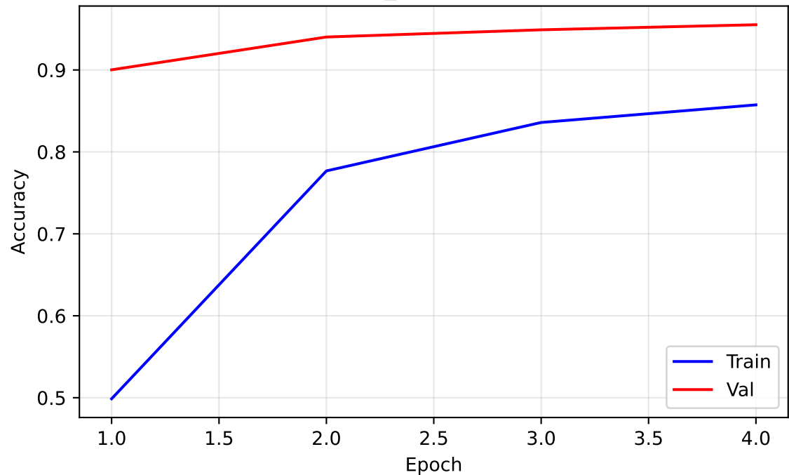
exp4_drop07 - Acc
