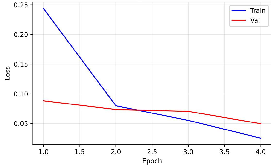
exp4_none - Loss
