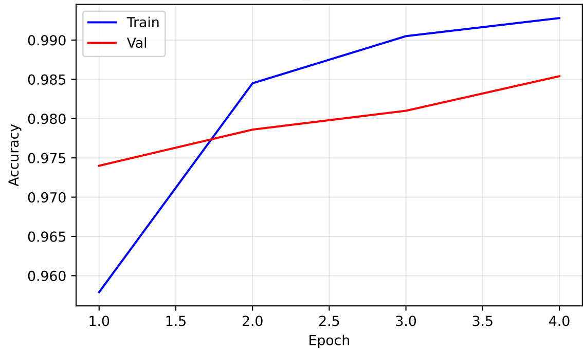
exp4_none - Acc
