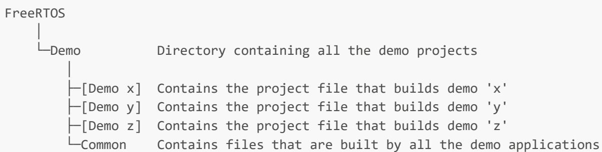
Figure 2.4 The demo directory hierarchy
