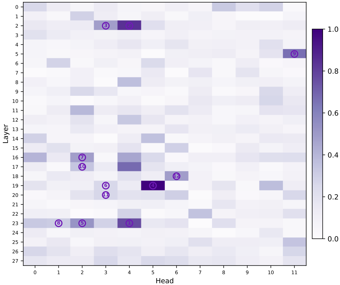
DeepSeek-R1-Distill-Qwen-1.5B_vs_Qwen2.5-1.5B: normalized relative difference
