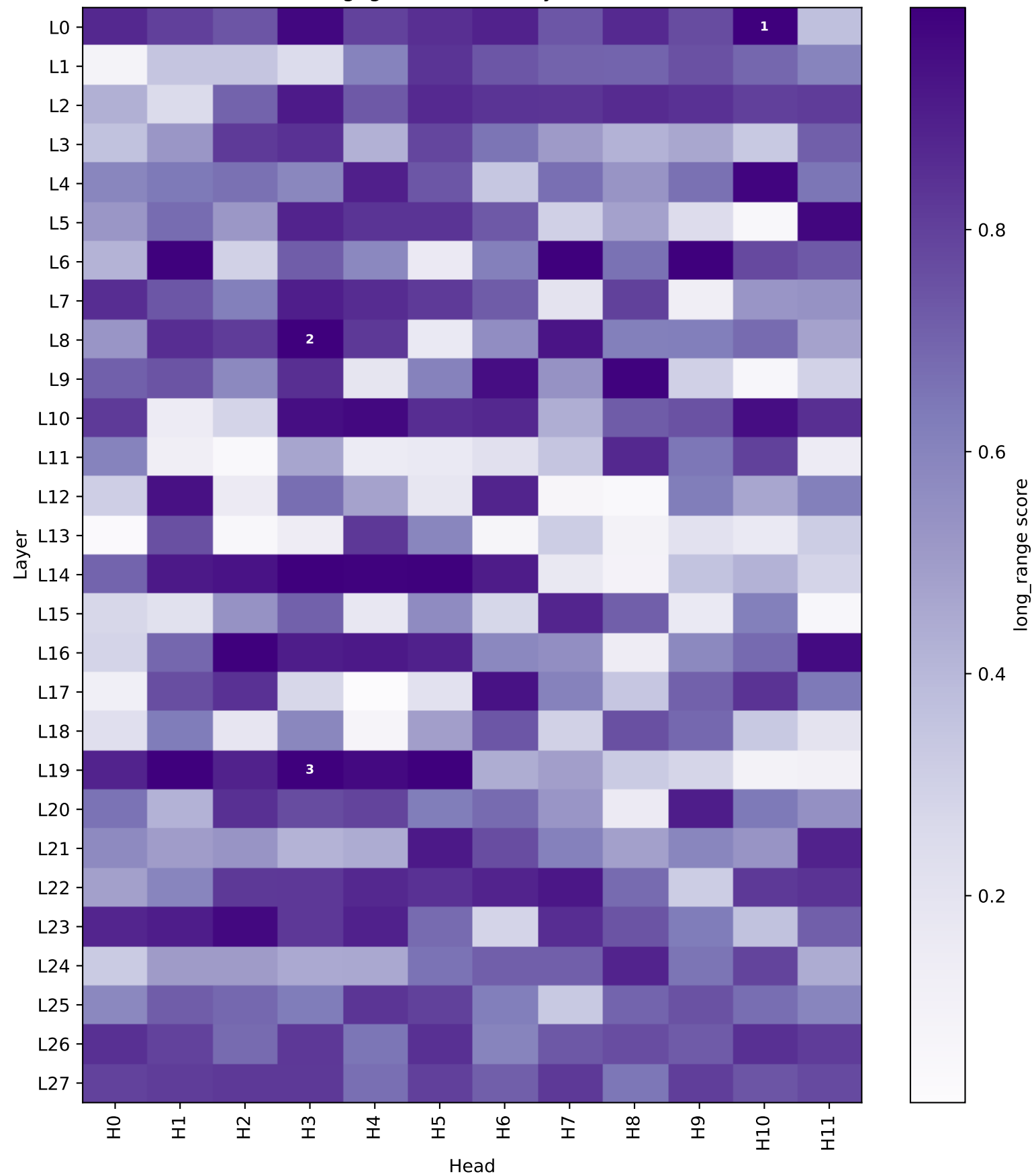
Layer x Head Importance: long_range Scoring ignores first 1 key column(s)
