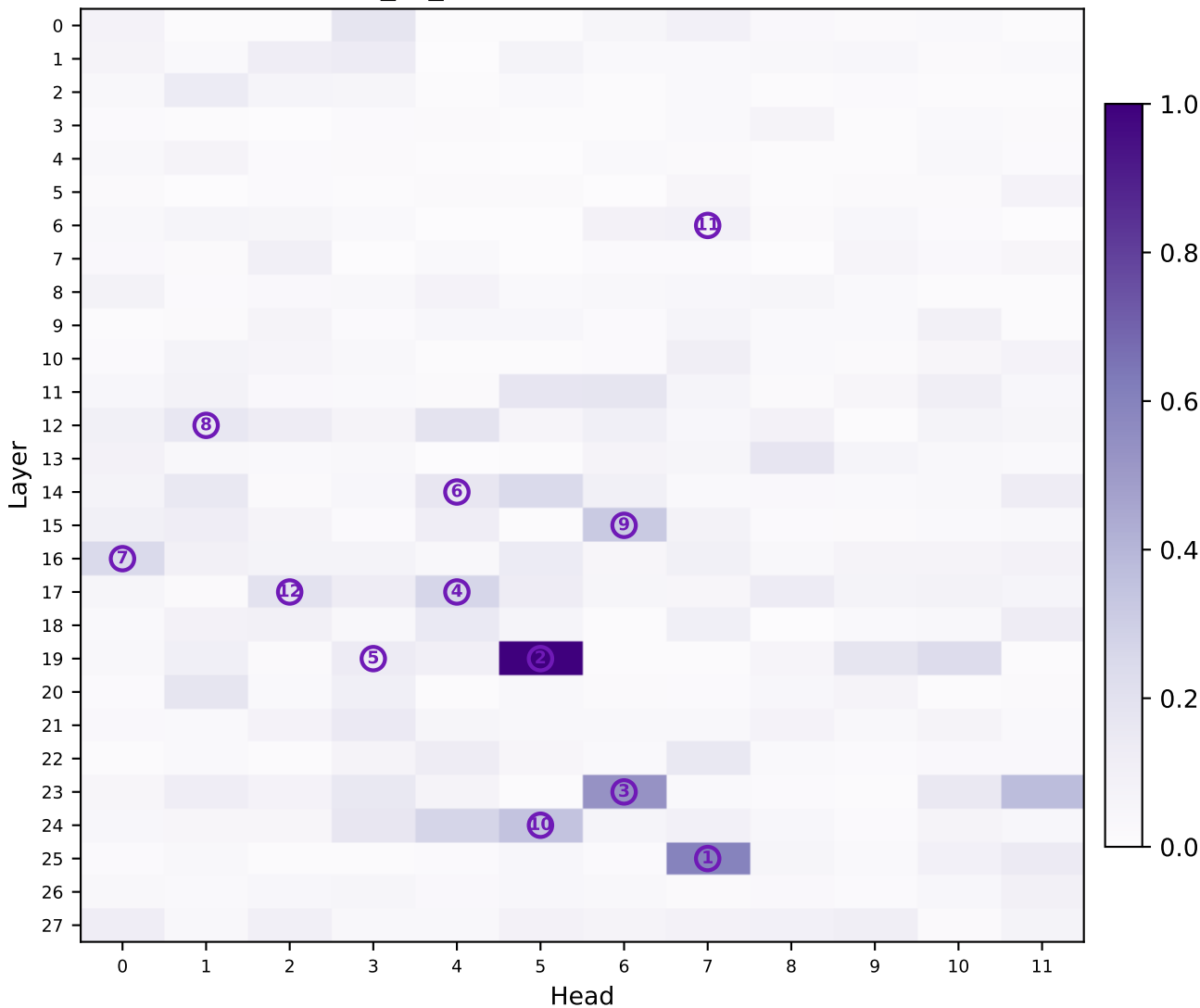
Qwen2.5-1.5B-Instruct_vs_Qwen2.5-1.5B: normalized relative difference
