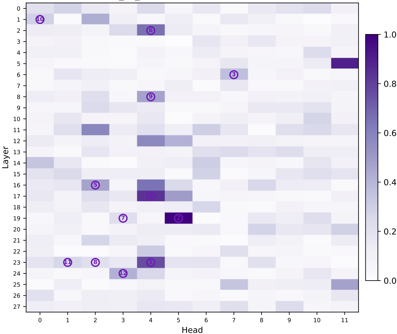
Qwen2.5-1.5B-Math_vs_Qwen2.5-1.5B: normalized relative difference
