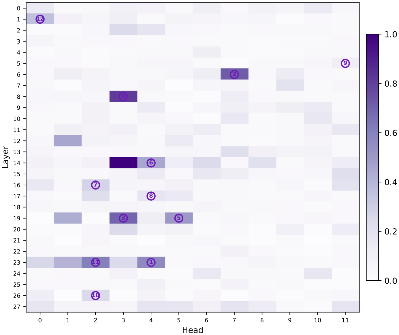
Qwen2.5-1.5B-Math-Instruct_vs_Qwen2.5-1.5B: normalized absolute salience
