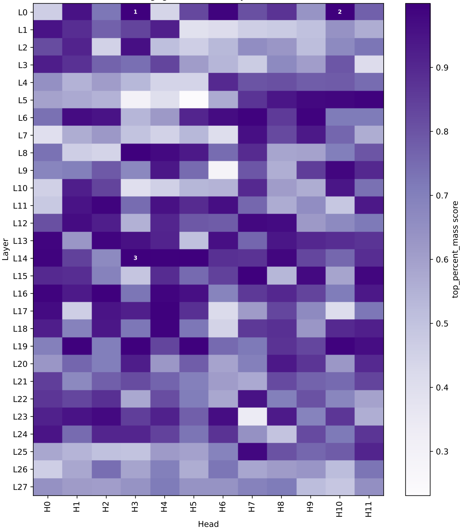
Layer x Head Importance: top_percent_mass Scoring ignores first 1 key column(s)
