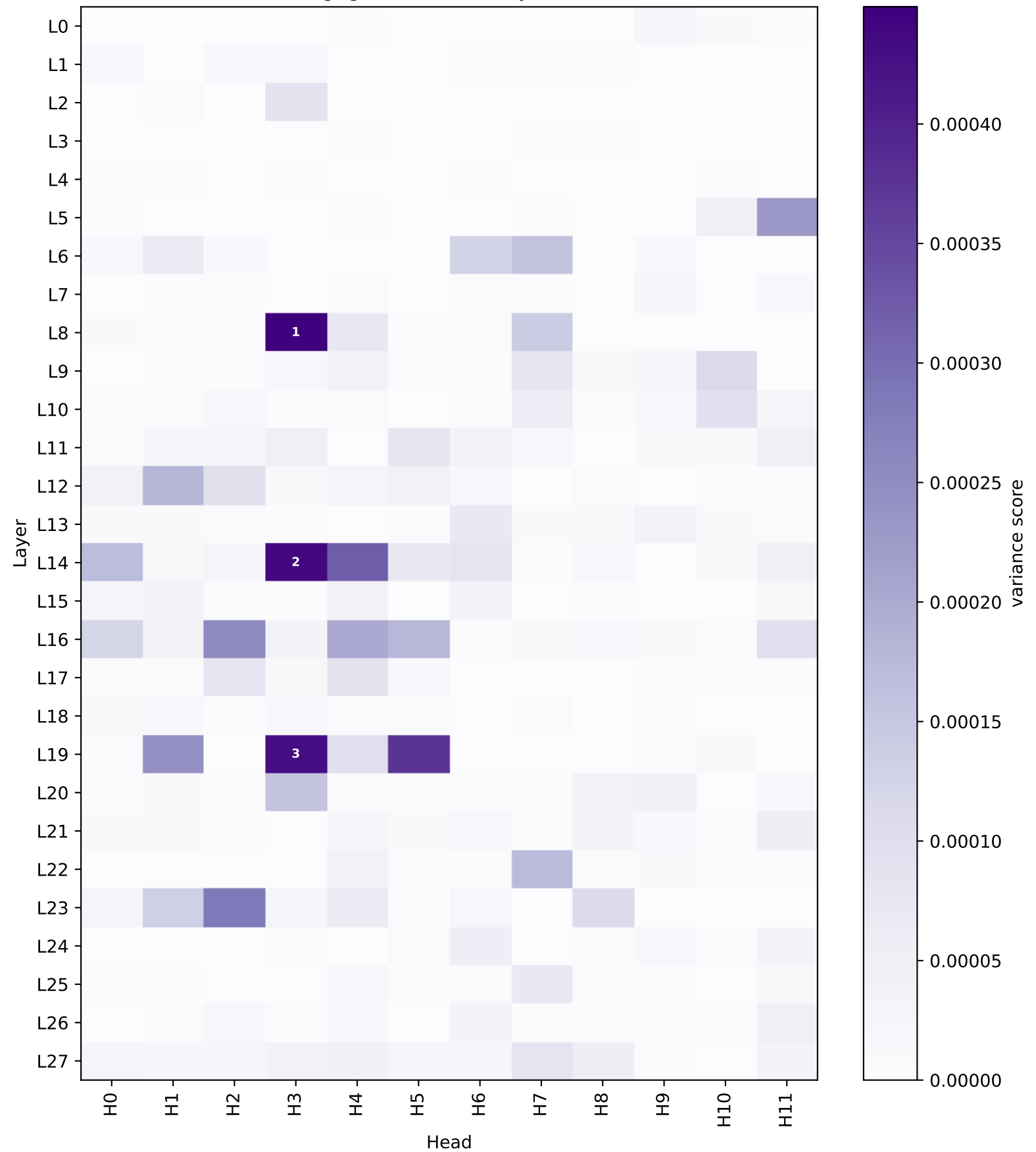
Layer x Head Importance: variance Scoring ignores first 1 key column(s)
