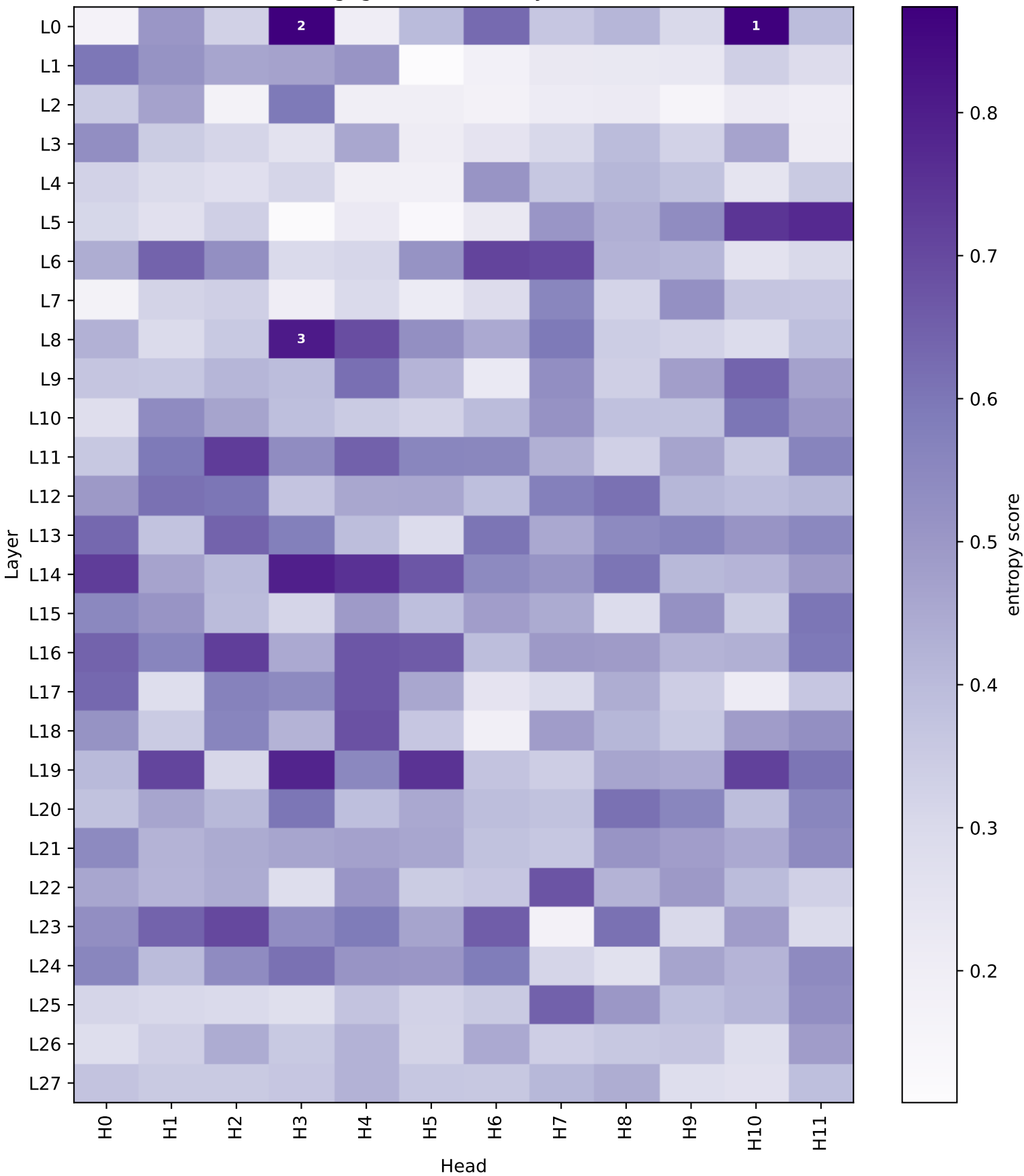
Layer x Head Importance: entropy Scoring ignores first 1 key column(s)
