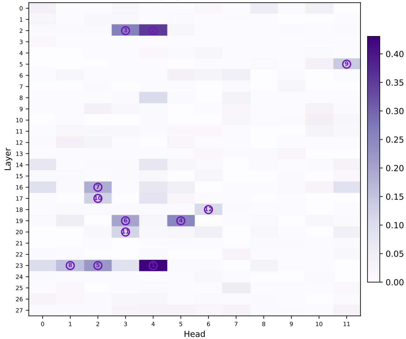
DeepSeek-R1-Distill-Qwen-1.5B_vs_Qwen2.5-1.5B: distinctive selection score
