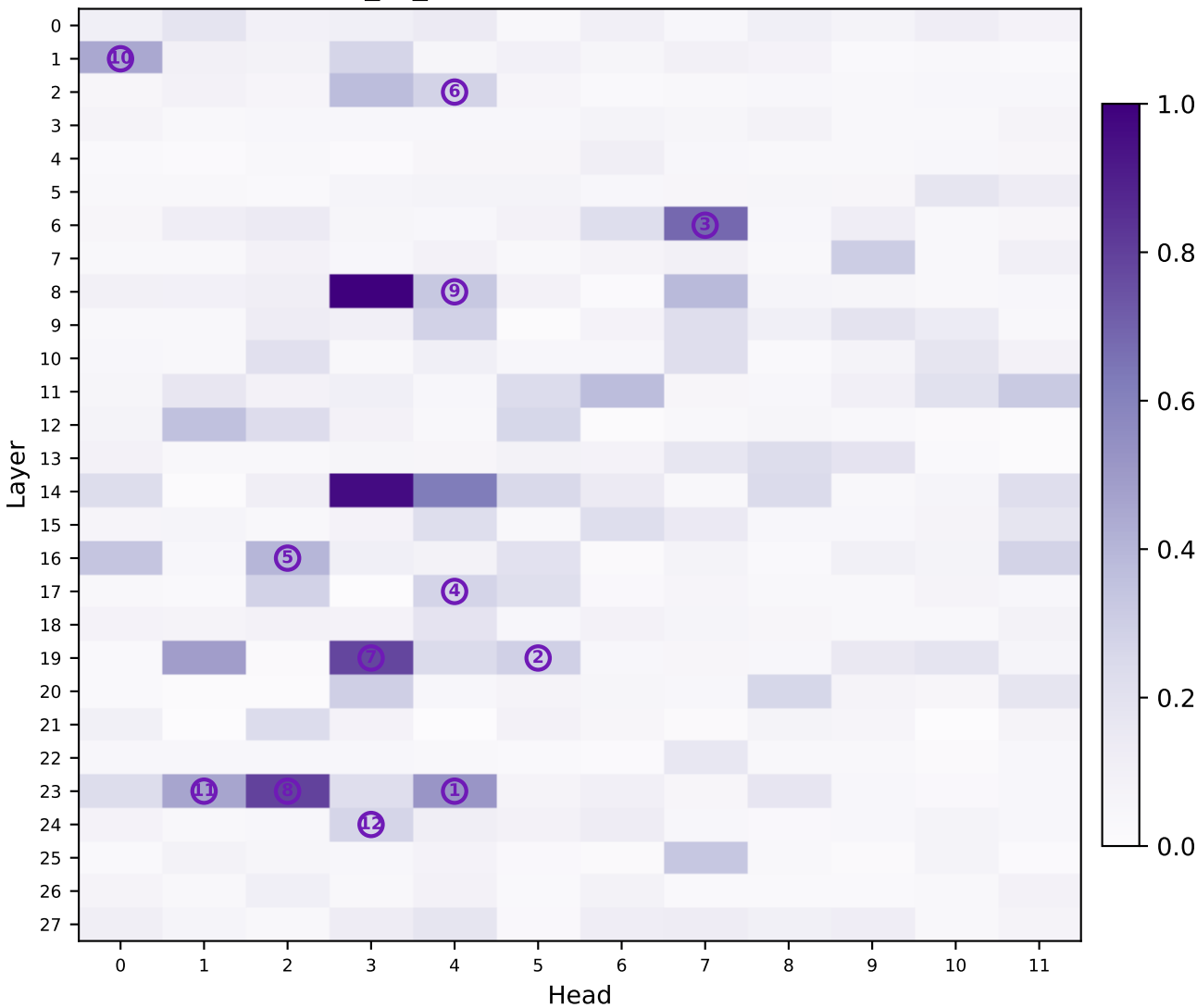
Qwen2.5-1.5B-Math_vs_Qwen2.5-1.5B: normalized absolute salience
