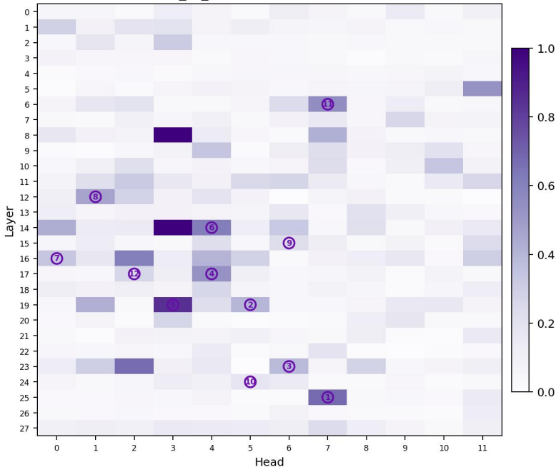
Qwen2.5-1.5B-Instruct_vs_Qwen2.5-1.5B: normalized absolute salience
