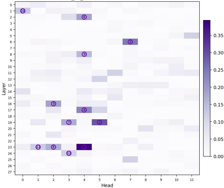
Qwen2.5-1.5B-Math_vs_Qwen2.5-1.5B: distinctive selection score
