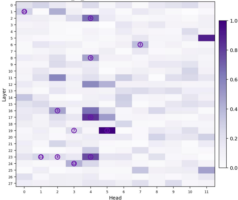
Qwen2.5-1.5B-Math_vs_Qwen2.5-1.5B: normalized relative difference
