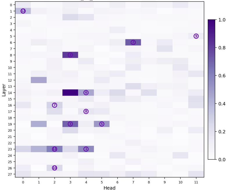
Qwen2.5-1.5B-Math-Instruct_vs_Qwen2.5-1.5B: normalized absolute salience
