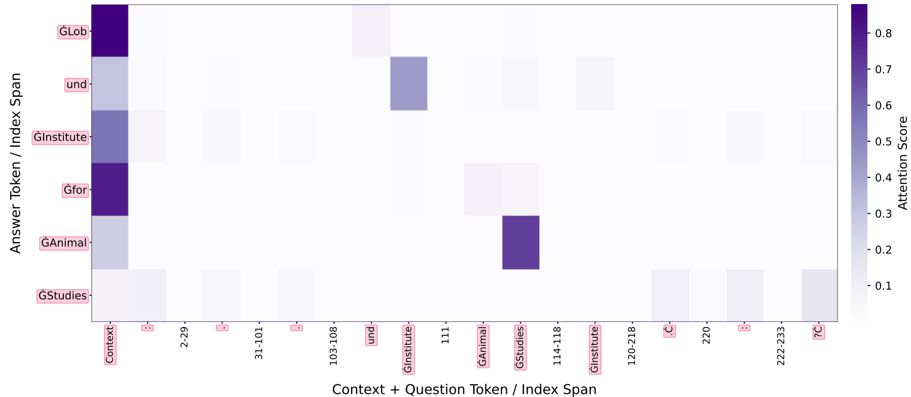
Qwen2.5-1.5B: L23 H4 answer -> context/question
