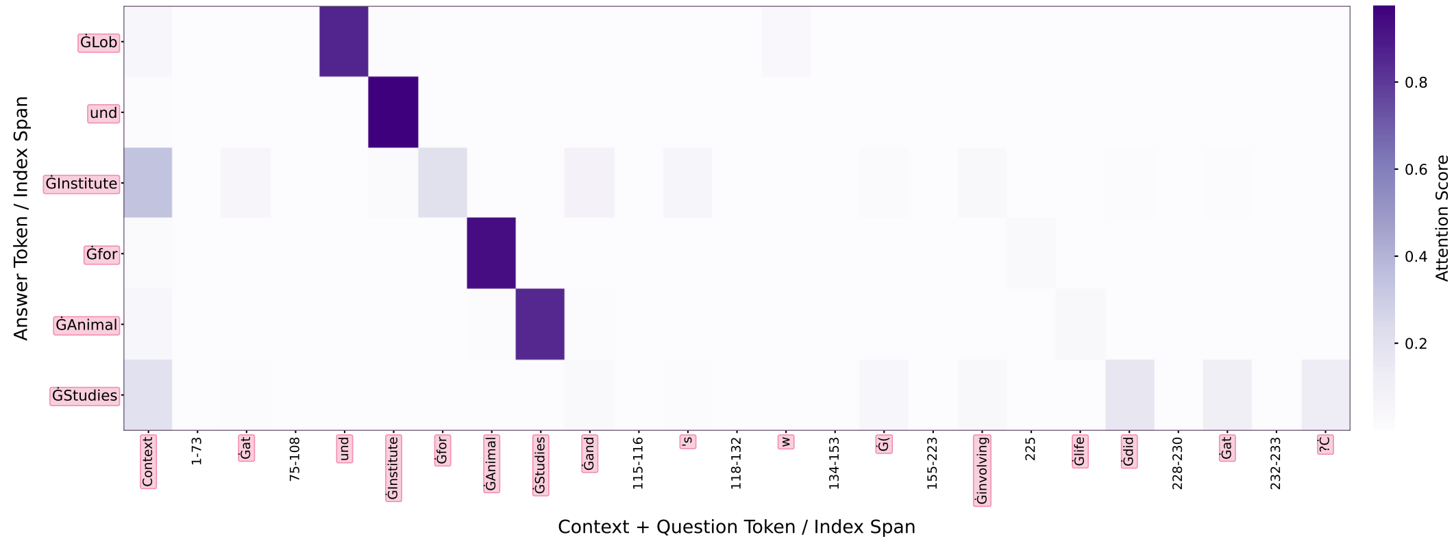
Qwen2.5-1.5B-Math-Instruct: L23 H4 answer -> context/question
