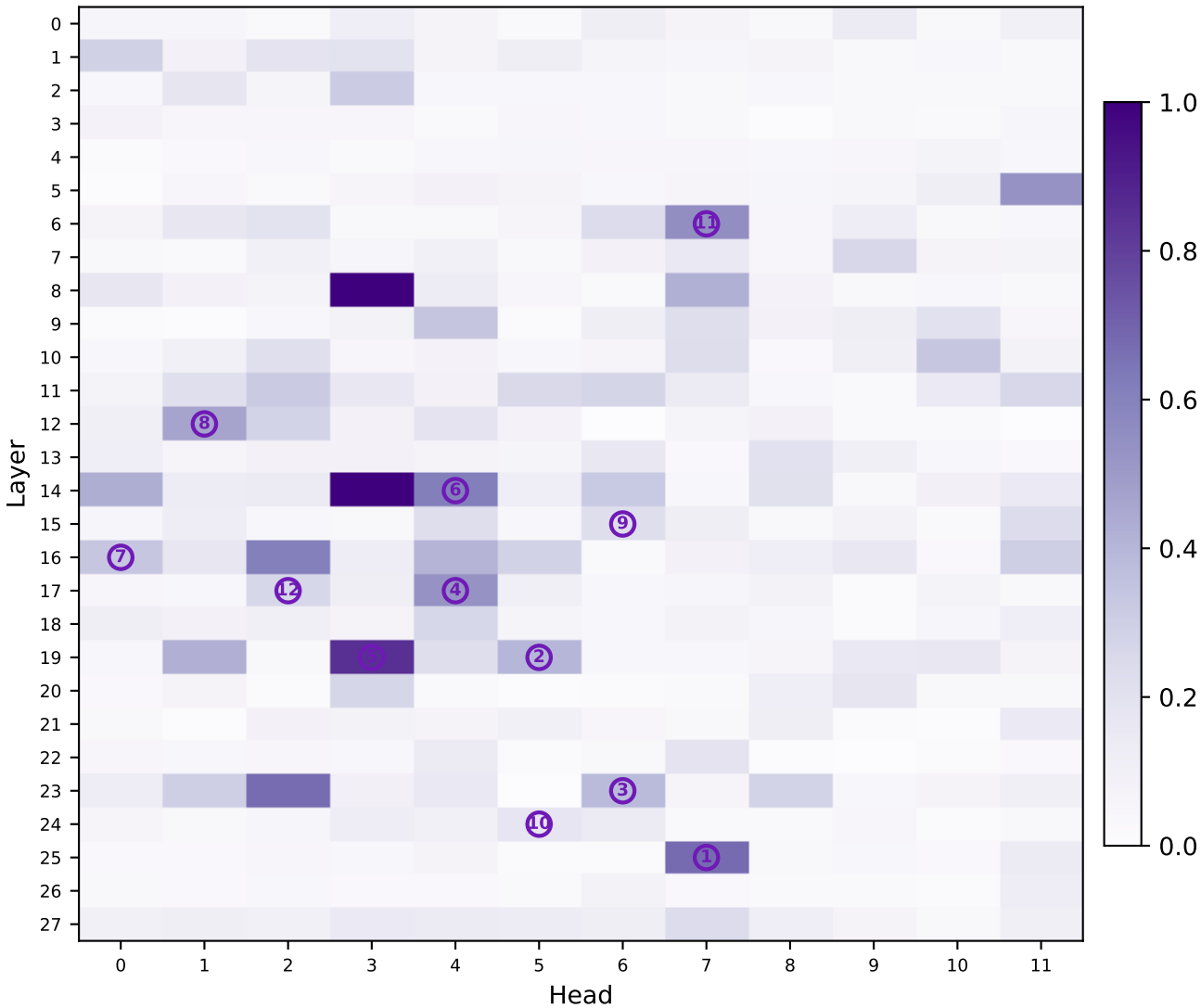
Qwen2.5-1.5B-Instruct_vs_Qwen2.5-1.5B: normalized absolute salience
