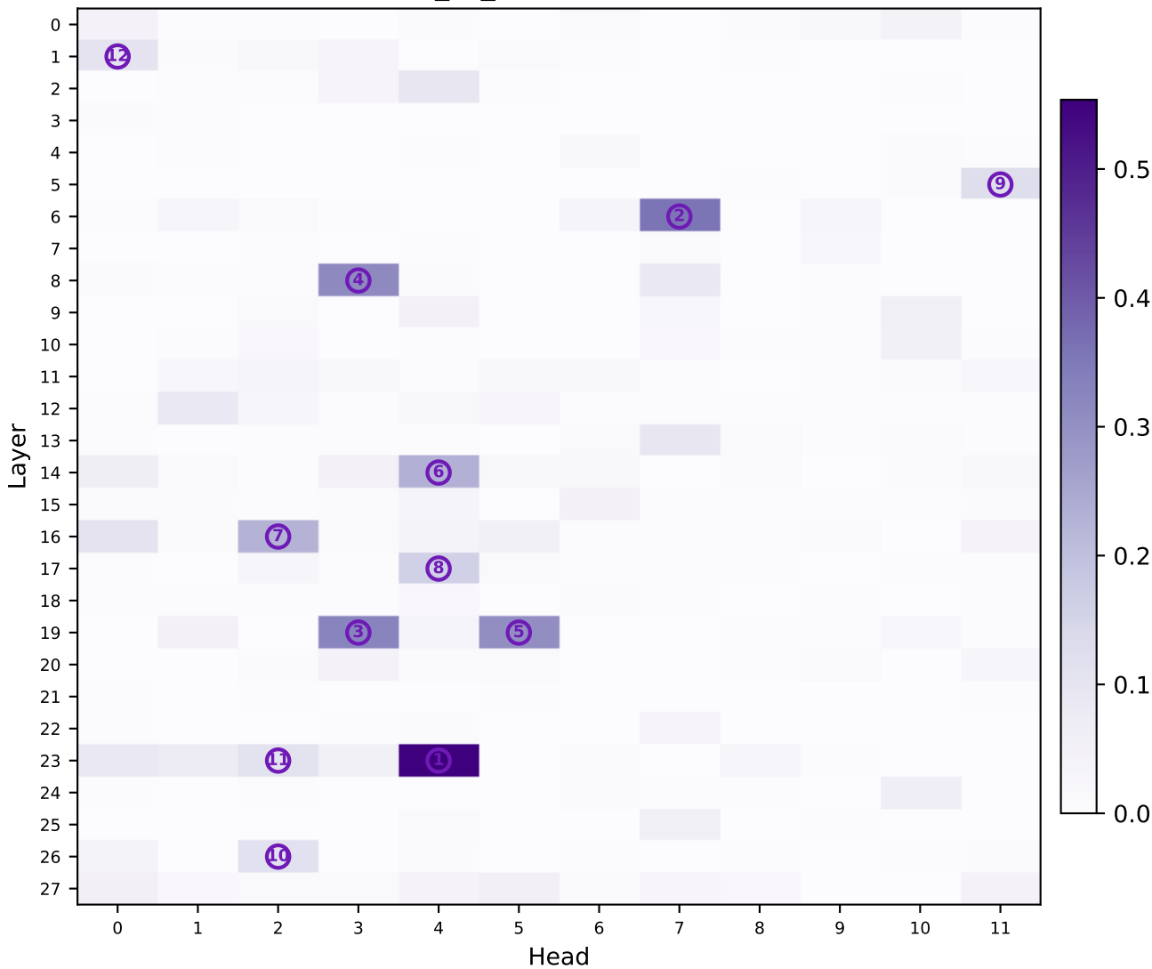
Qwen2.5-1.5B-Math-Instruct_vs_Qwen2.5-1.5B: distinctive selection score
