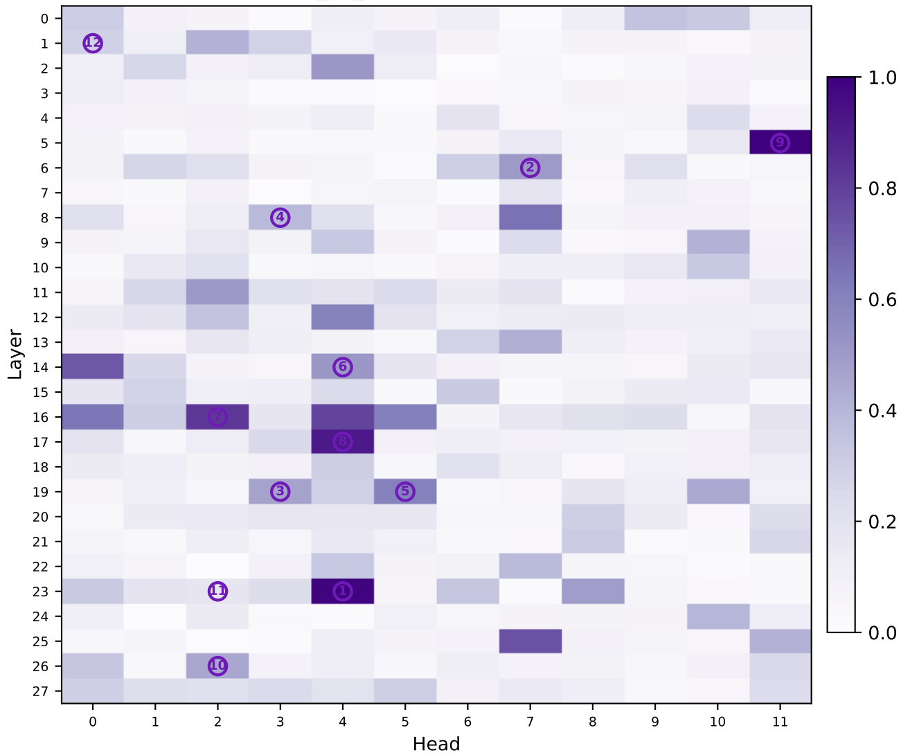
Qwen2.5-1.5B-Math-Instruct_vs_Qwen2.5-1.5B: normalized relative difference
