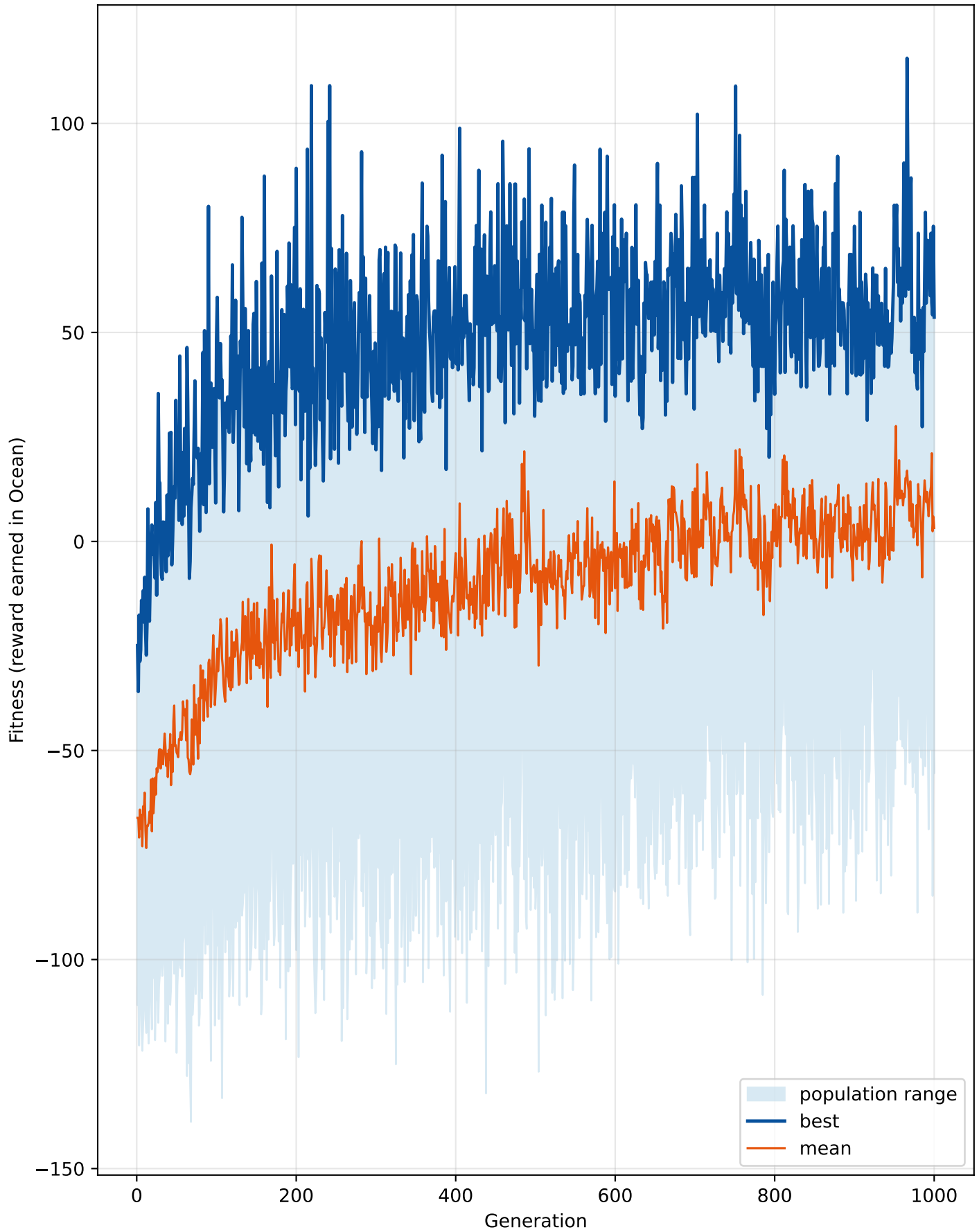
Fitness over generations
