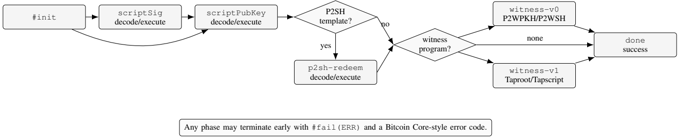
Fig. 3. Simplified phase machine for script verification. The curved #init-to-scriptPubKey edge is the empty-scriptSig path; the witness branch targets either v0 or v1 execution. The actual K rules include additional side conditions such as push-only checks, WITNESS_MALLEATED, WITNESS_UNEXPECTED, clean-stack checks, witness-program length checks, and Taproot control-block validation.
