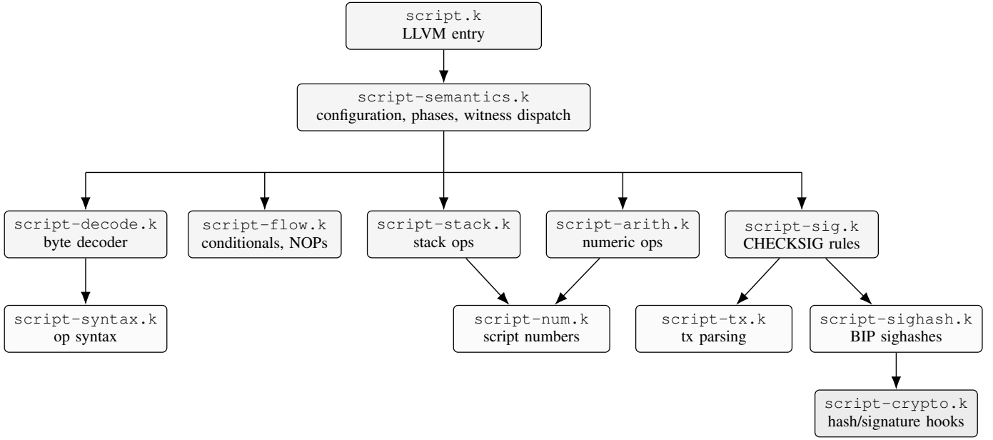
Fig. 1. High-level organization of the executable K definition. The core configuration and phase machinery live in script- semantics.k ; opcode families are separated into smaller modules, while cryptographic primitives are delegated to native hooks.
