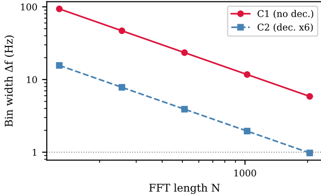
(a) Resolution vs FFT length
