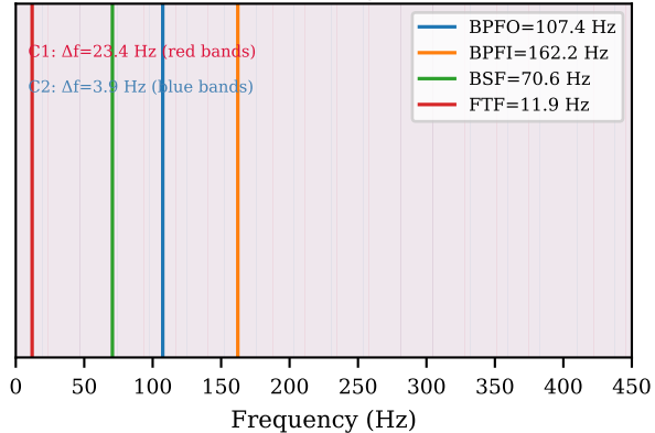
(b) Fault lines vs bin grids (N=512)
