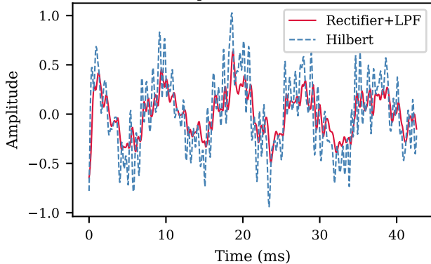
(a) Envelope (time domain, seed 0)
