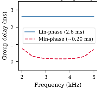
(b) Passband group delay
