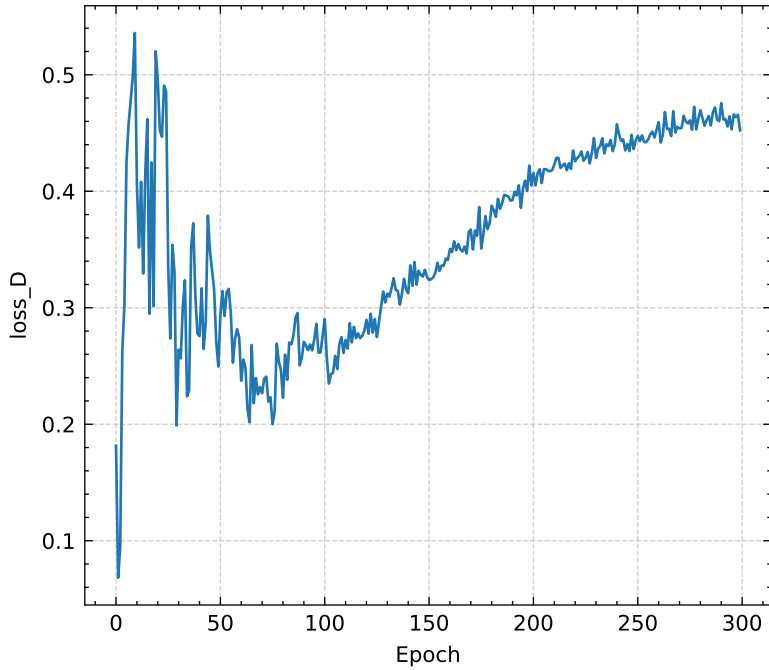
loss_D vs Epoch
