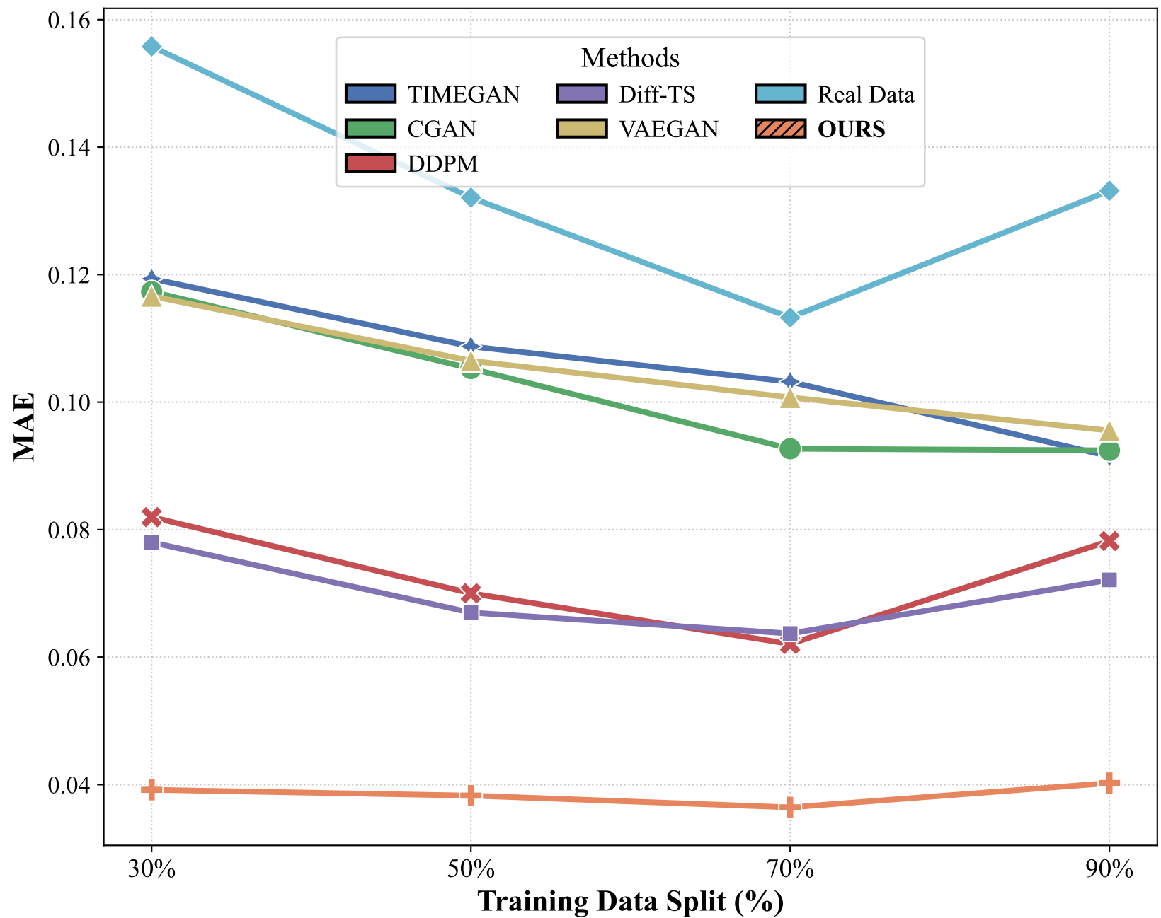
MAE Trends with Increasing Training Data
