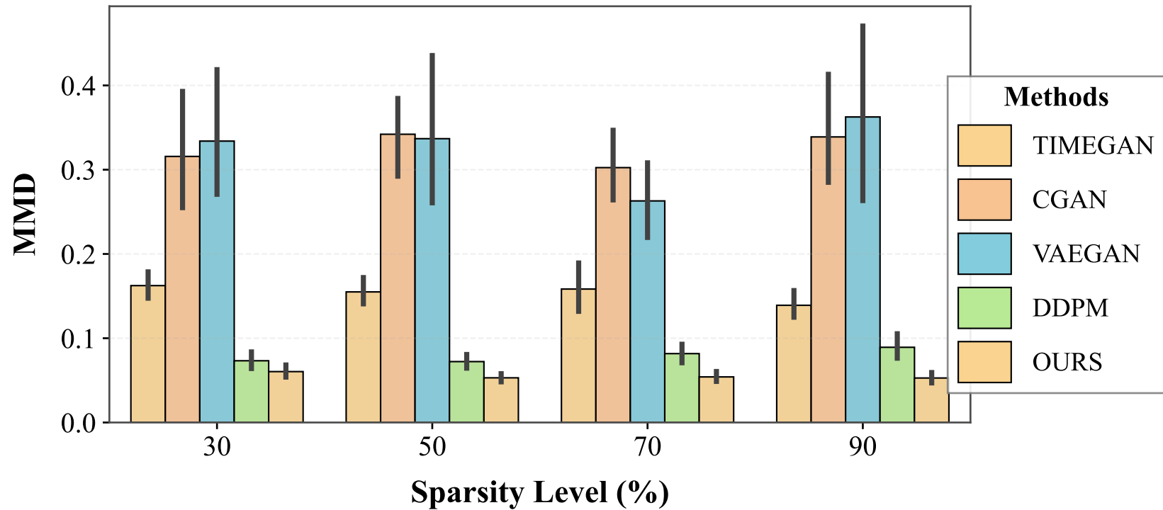
Distribution Distance to Original Data (MMD)
