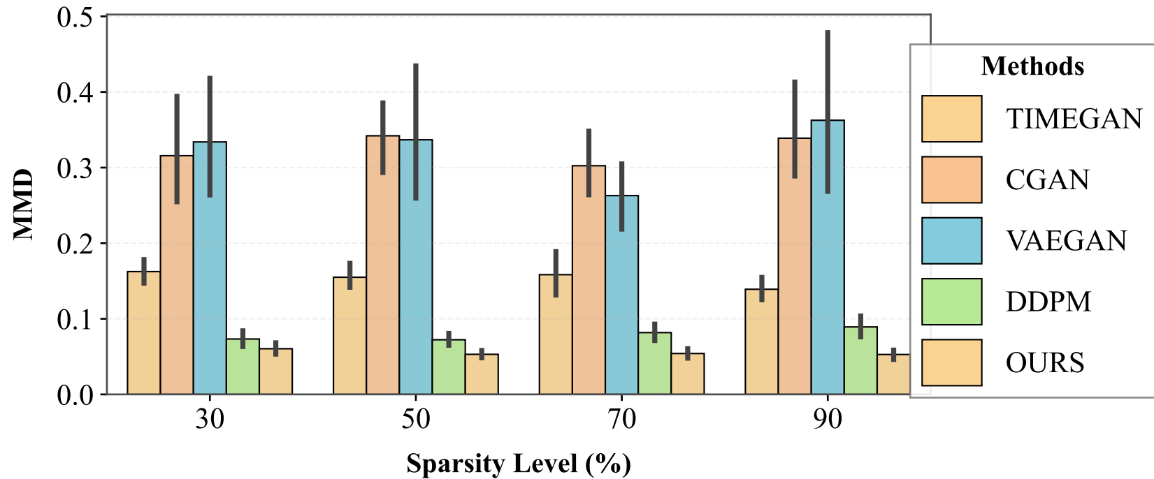
Distribution Distance to Original Data (MMD)
