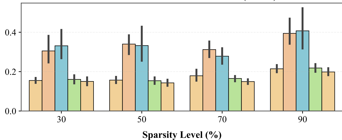
Distribution Distance to Test Data (MMD)
