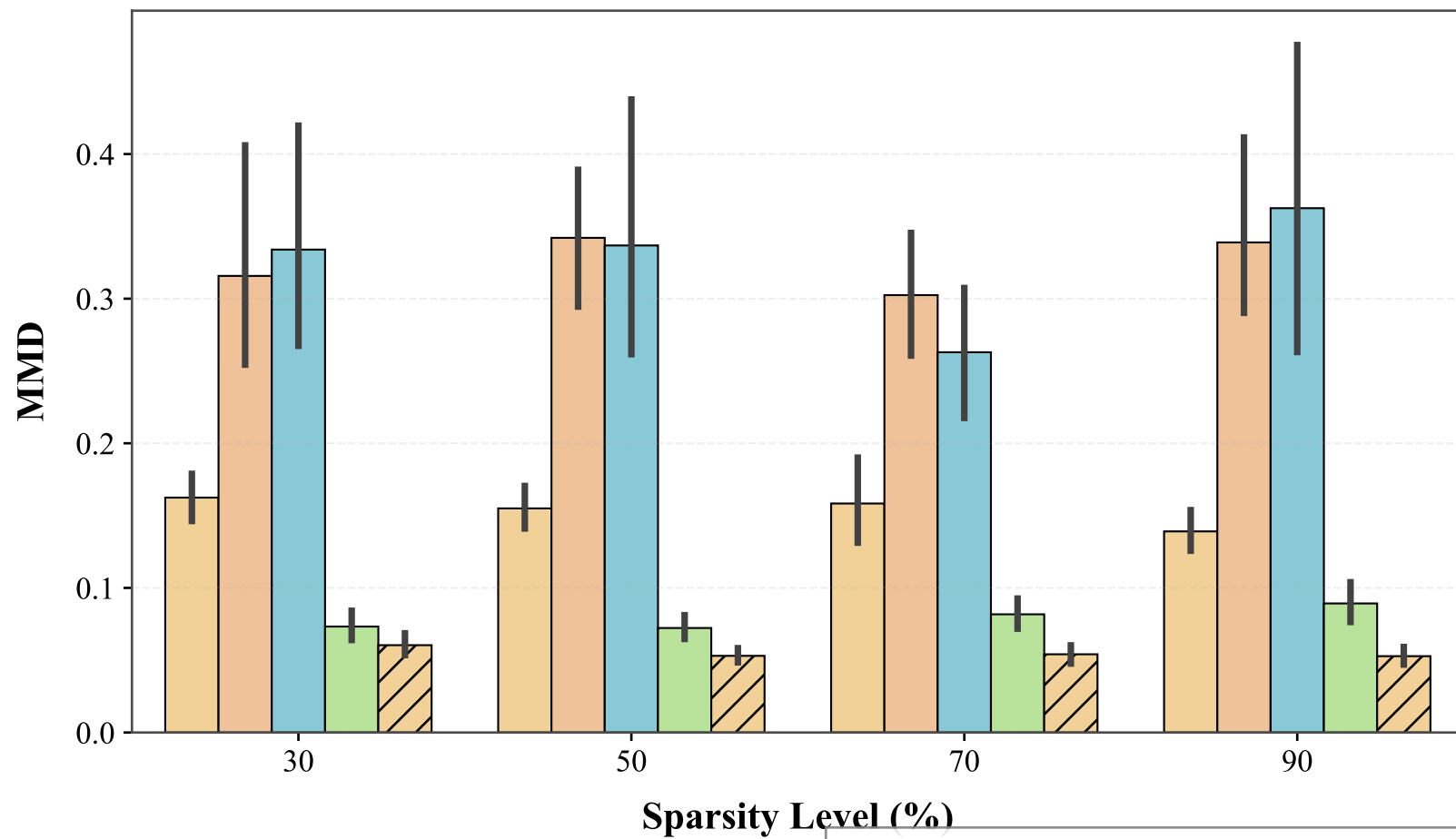
Distribution Distance to Original Data (MMD)
