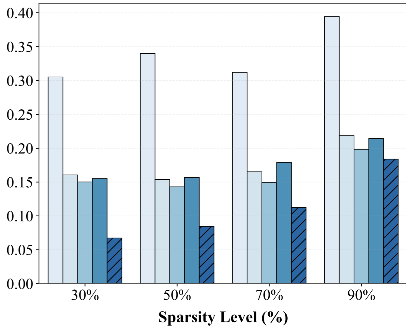
Distribution Distance to Test Data (MMD)
