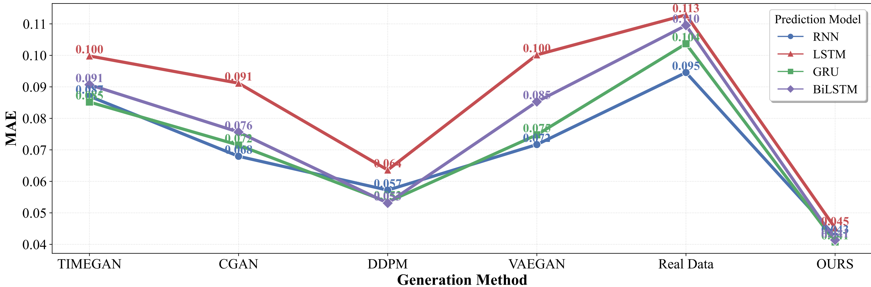
MAE Comparison Across Different Models (70% Training Data)
