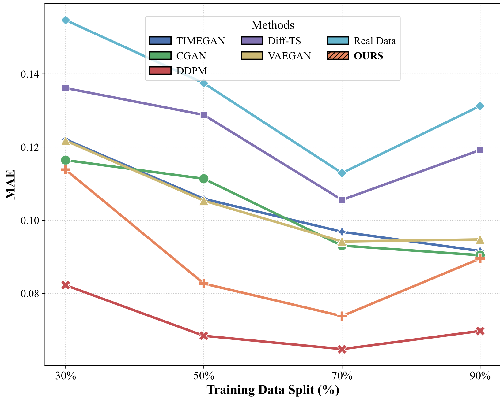
MAE Trends with Increasing Training Data
