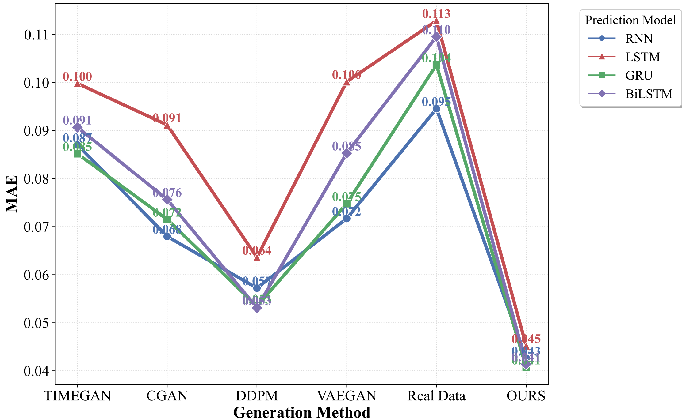
MAE Comparison Across Different Models (70% Training Data)
