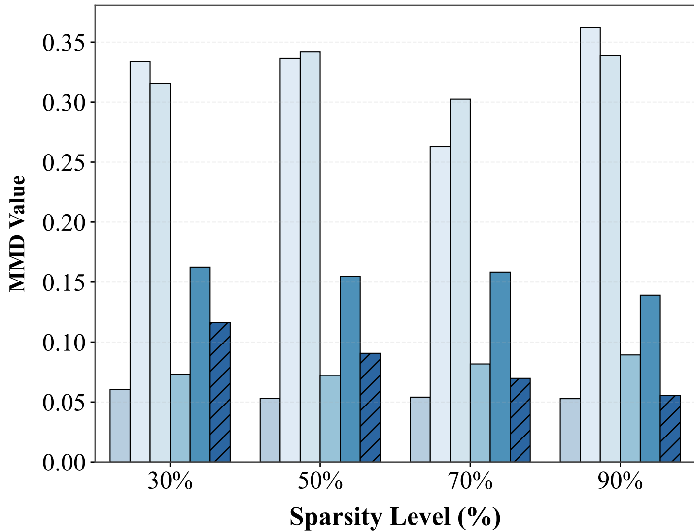
Distribution Distance to Original Data (MMD)
