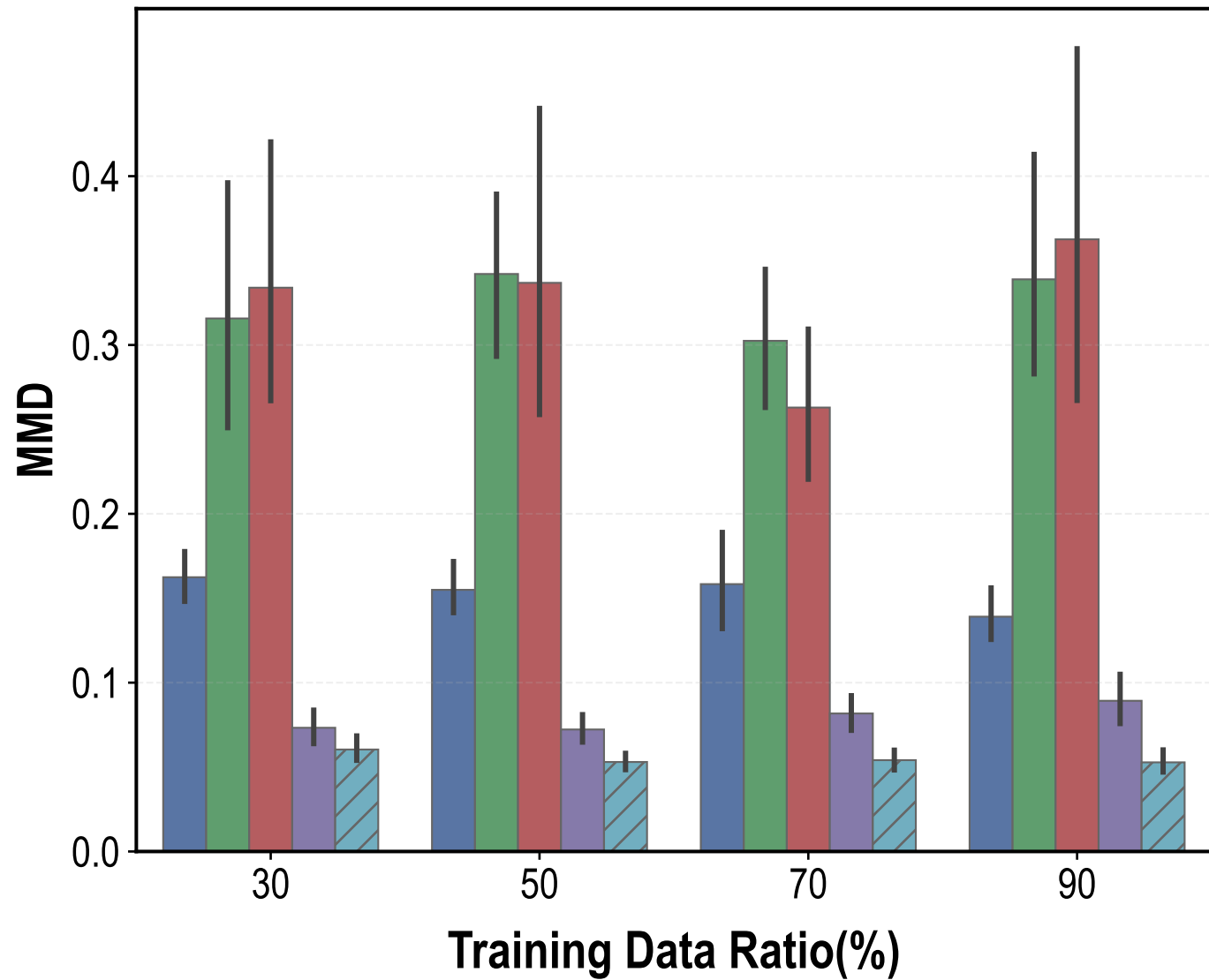
Distribution Distance to Original Data (MMD)
