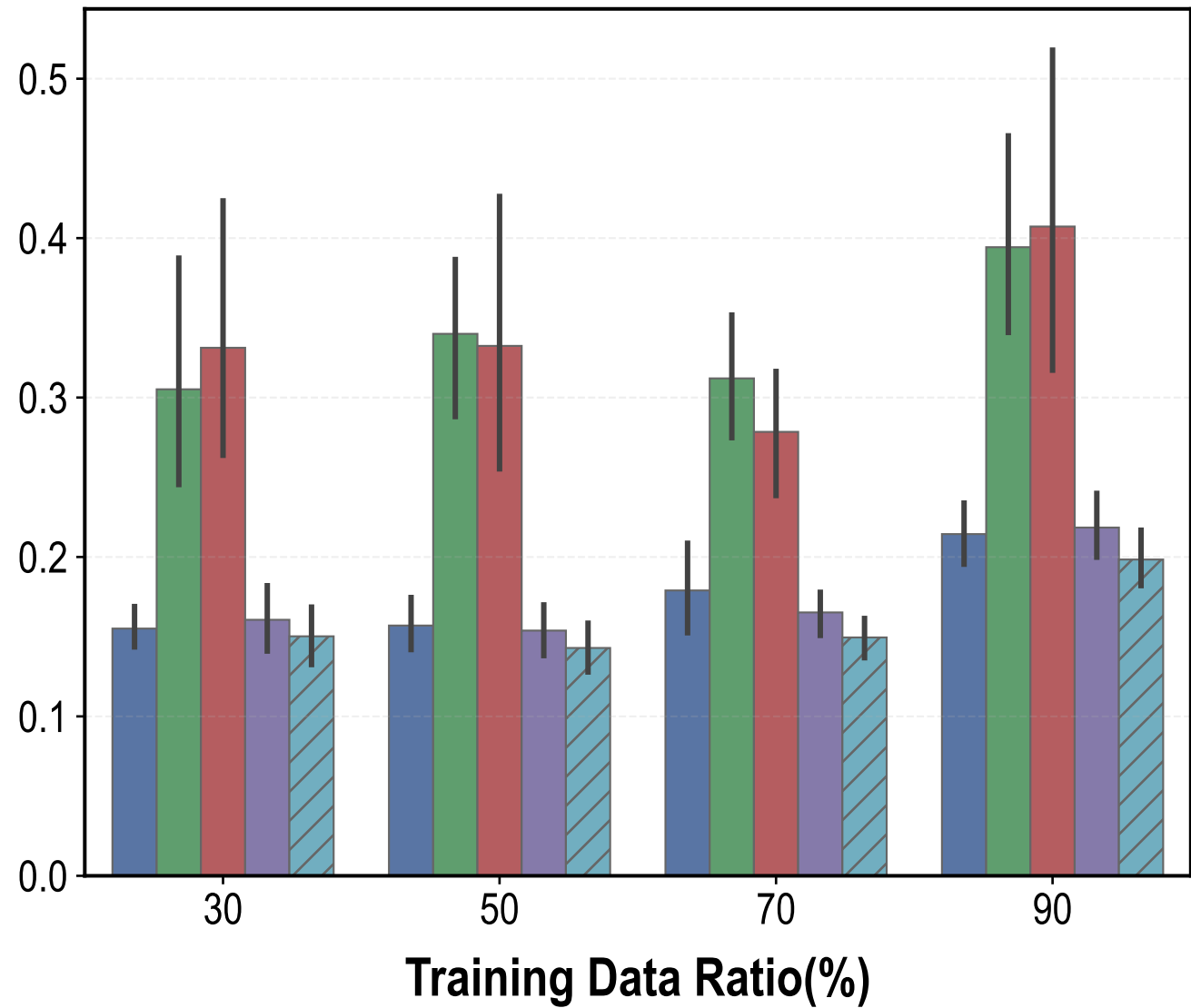
Distribution Distance to Test Data (MMD)
