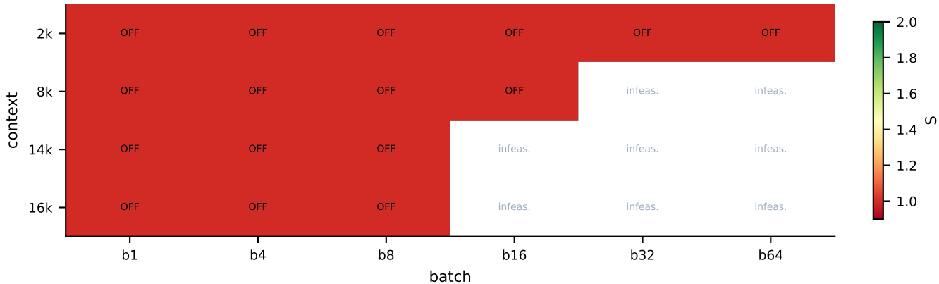
moe: predicted per-cell winner (Stage A; S vs AR)
