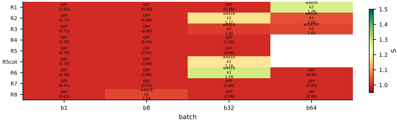
moe: real-data winner per dataset x batch (Stage B; S vs AR)
