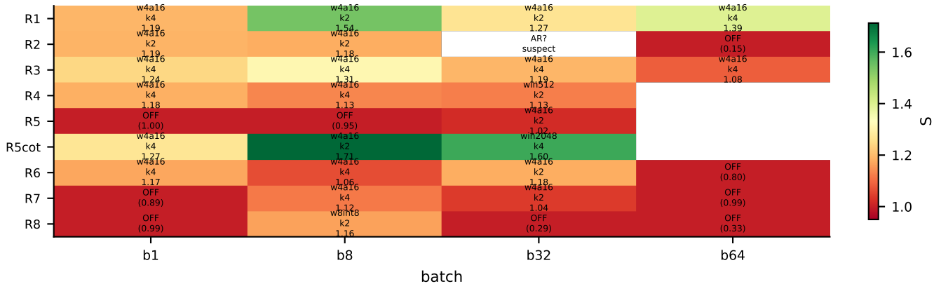
llama: real-data winner per dataset x batch (Stage B; S vs AR)
