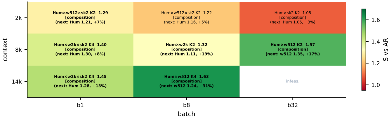
dense: C2 winner per cell over singles + compositions (8/8 cells won by a composition)
