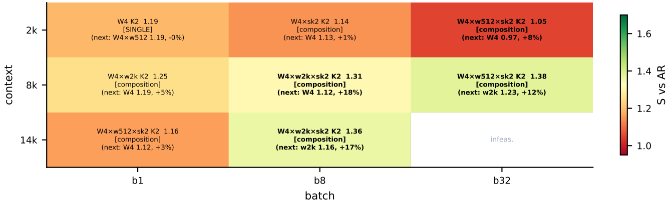
llama: C2 winner per cell over singles + compositions (7/8 cells won by a composition)
