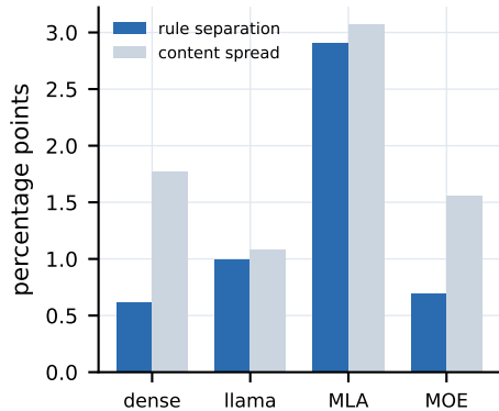
rule choice vs content noise
