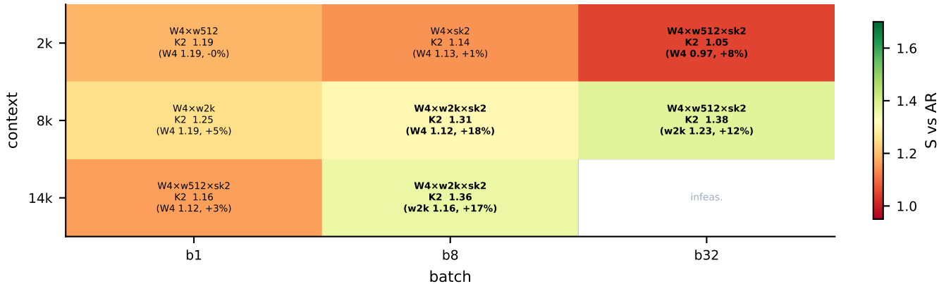
llama: C2 winning COMPOSITION per cell (displaced single in parentheses)
