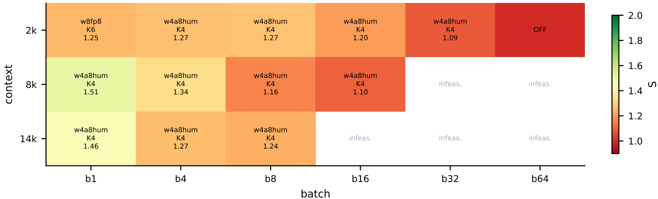
q3_32b: predicted per-cell winner (Stage A; S vs AR)
