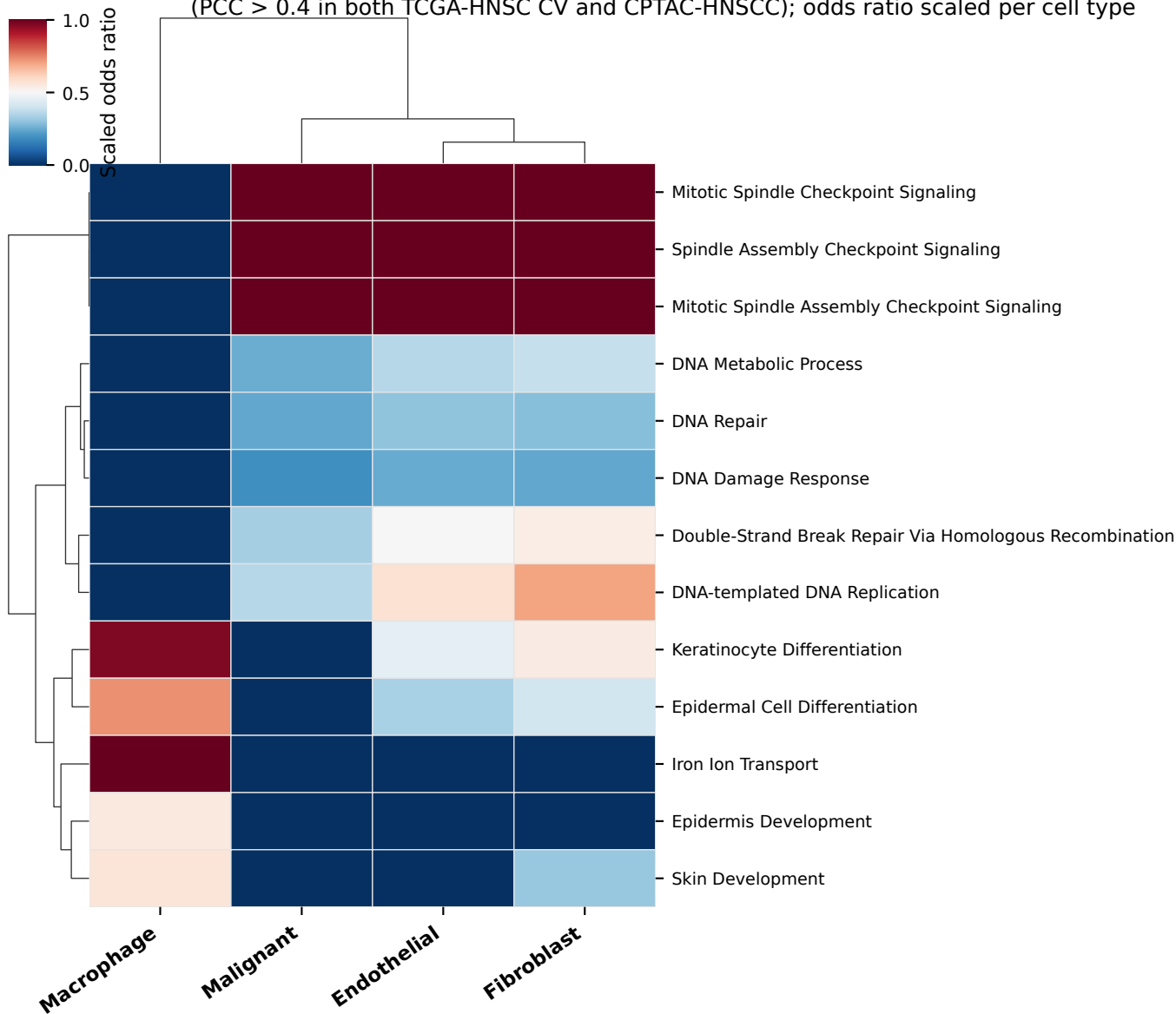
Figure 5. GO(BP) enrichment of cross-cohort robustly-predicted genes (PCC > 0.4 in both TCGA-HNSC CV and CPTAC-HNSCC); odds ratio scaled per cell type
