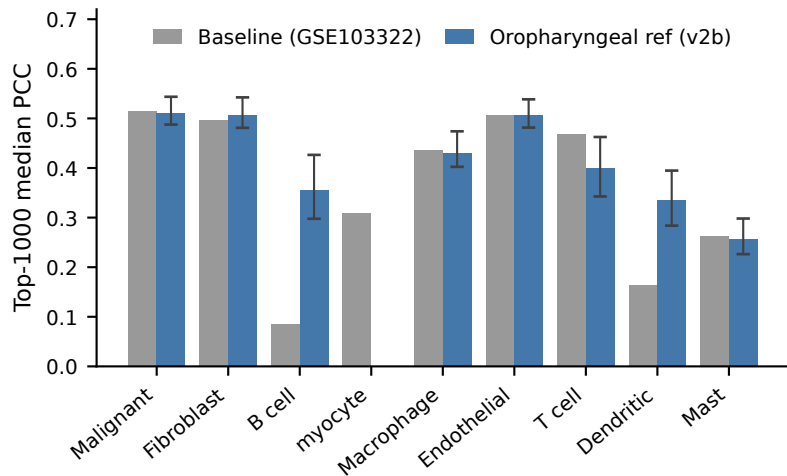
a. Reference swap rescues B-cell / dendritic prediction
