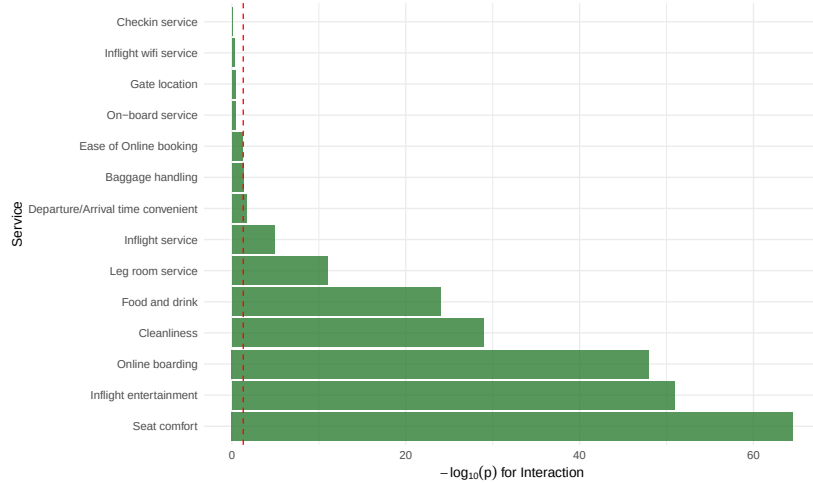
Figure 17: Figure 3.8 ANOVA Interaction Effects
