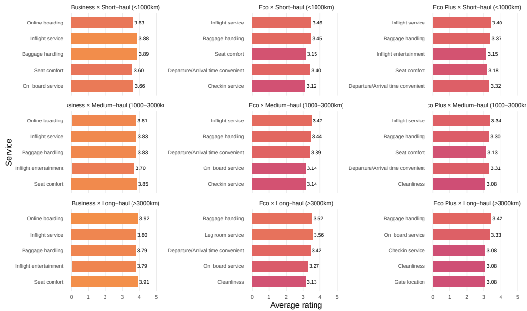
Figure 15: Figure 3.6 Top-5 Services by Cabin Class × Flight Distance
