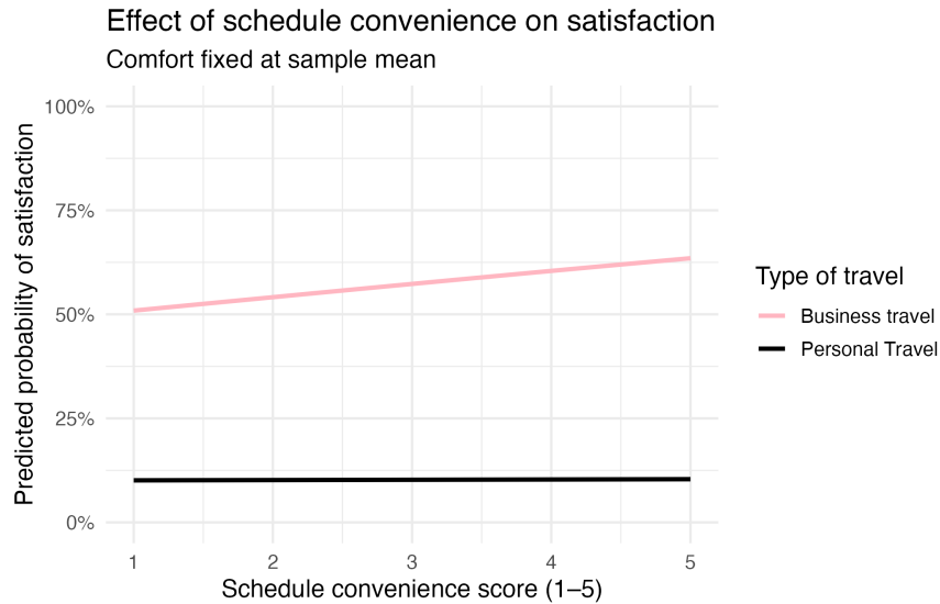
Figure 12: Figure 3.3.5 Effect of schedule convenience on satisfaction
