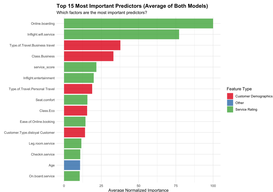
Figure 22: Figure 5.5 Top 15 most important predictors (average of both models)
