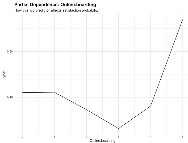
Figure 24: Figure 5.7 Partial dependence plot for Online boarding (top predictor)
