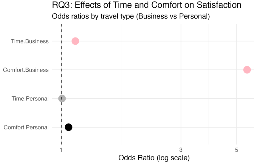
Figure 11: Figure 3.3.4 Effects of time and comfort on satisfaction: Odds ratios by travel type
