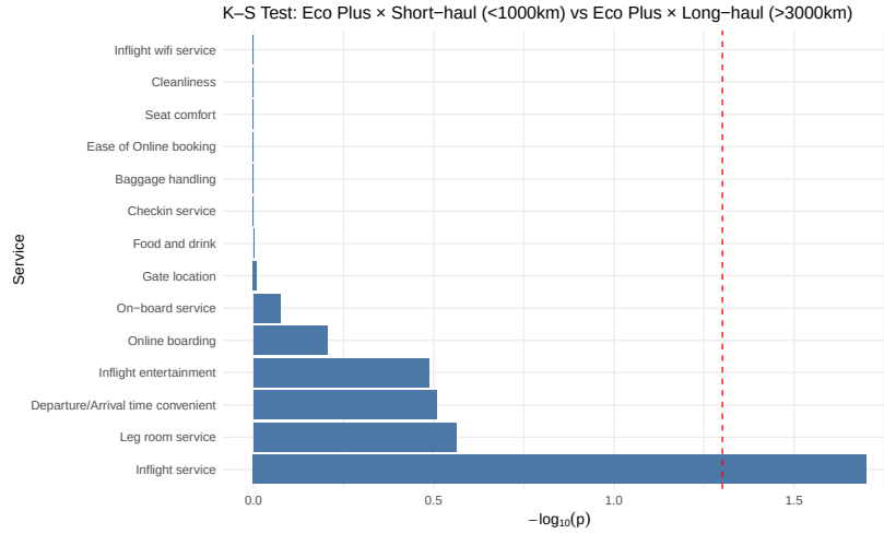
Figure 16: Figure 3.7 K–S Test Results (Eco Plus Short vs. Long)
