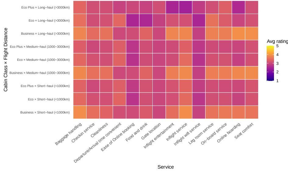
Figure 14: Figure 3.5 Heatmap of Average Ratings
