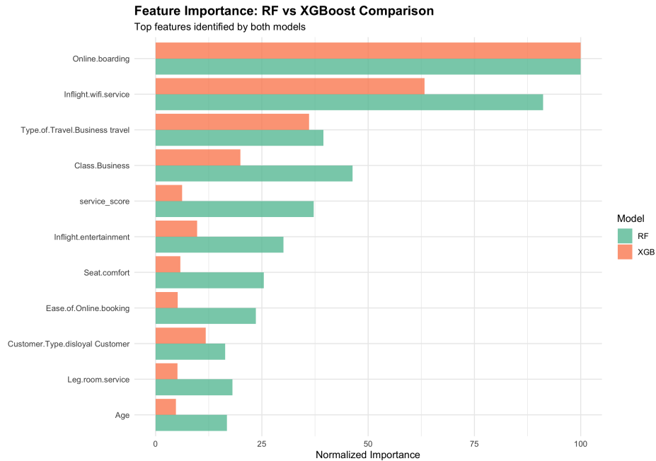
Figure 23: Figure 5.6 Feature importance: RF vs XGBoost comparison
