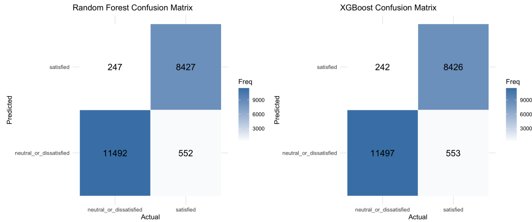
Figure 21: Figure 5.4 Confusion matrices for Random Forest and XGBoost
