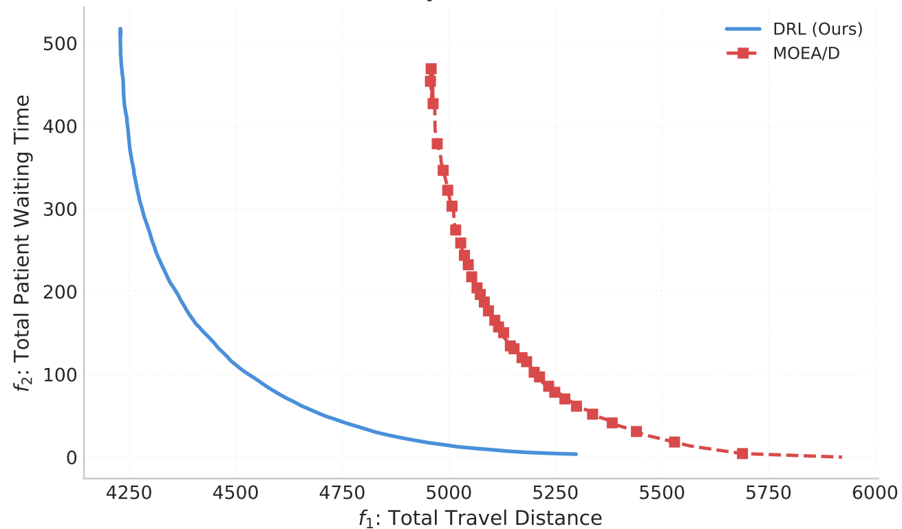
Pareto Front Comparison — HHCRSP n=100
