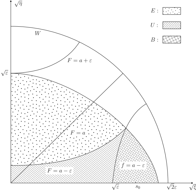
Figure C.2: U hatched; f^{-1}((-\infty, a - \varepsilon)) \cap U double-hatched
