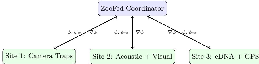
Figure 1: ZooFed federated learning architecture.
