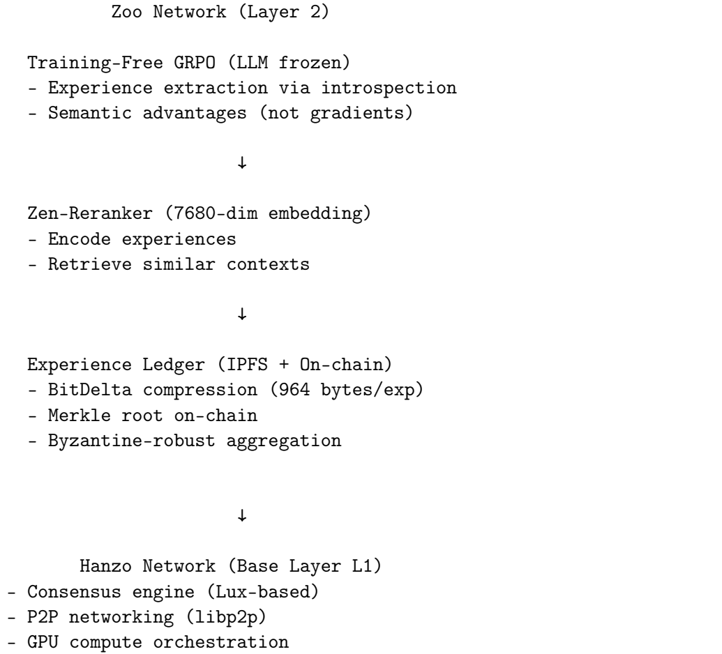
Figure 1: Zen-Reranker integration in Zoo Network architecture
