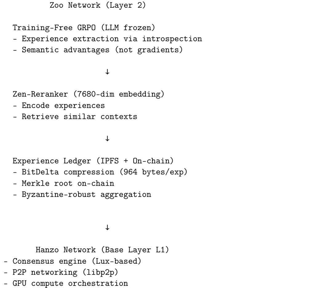
Figure 1: Zen-Reranker integration in Zoo Network architecture
